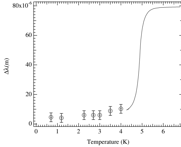
Figure 6. Change in penetration depth versus temperature at zero field in \lambda -(BETS) 2 GaCl 4 . Note that the cryostat used could only provide controlled, slow sweeps of temperature down to 4.2 K (data shown as a continuous curve). Below this, data are recorded at fixed, stable temperatures (points). The error bars on the points give typical uncertainties, valid across the whole temperature range shown.
