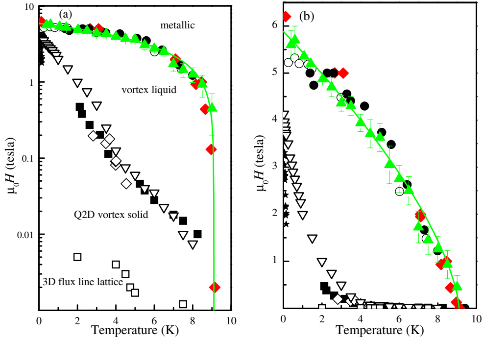
Figure 10. Critical fields in \kappa -(BEDT-TTF) 2 Cu(NCS) 2 , plotted on logarithmic (a) and linear (b) field scales. The data for H_{c2} comprise filled triangles (MHz penetration data obtained using the apparatus described in the current paper [52]), filled circles (microwave penetration studies; reference [46]; errors in values of \mu_0 H_{c2} typically \pm 0.5 T), open circles (thermal conductivity data from reference [46]; errors not given) and shaded diamonds (magnetization data; the lowest-temperature point was determined by examining the attenuation of de Haas–van Alphen oscillations [53] and the higher-temperature points are from the scaling studies in reference [54]). The solid curve is proportional to (T_c - T)^{2/3} , with T_c = 9.1 K. The triangles show the irreversibility field from magnetization [53]; the filled squares and stars represent 2D melting from magnetometry and GHz studies [56] (see also the NMR data of reference [57]). The hollow squares are from muon-spin-rotation studies [55] and denote the 3D–2D transition.
