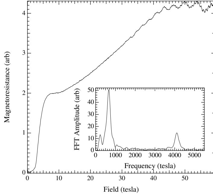
Figure 1. Resistance of a \lambda -(BETS) 2 GaCl 4 crystal as a function of magnetic field, applied parallel to the b^* -direction; the temperature is 340 mK. The inset shows a Fourier transform of the data after subtraction of the non-oscillatory background [1]. The peak at 650 T is associated with the \alpha -pocket; that at 4030 T is due to the breakdown ( \beta -) orbit which encompasses 100% of the Brillouin zone.
