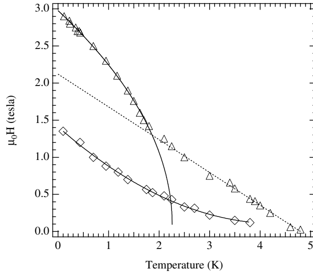
Figure 9. The notional phase diagram of \lambda -(BETS) 2 GaCl 4 showing the upper critical field (triangles) and H^* , marking the inflection points in the penetration depth (diamonds). The quasistatic field is applied parallel to b^* , i.e. perpendicular to the quasi-two-dimensional planes of the sample. Points from four different samples are shown, often overlaying each other. The upper solid curve is H_{c2} \propto (T^* - T)^{1/2} ; the dashed curve is H_{c2} \propto (T_{c2} - T) . The lower solid curve is a fit of the two-fluid model expression for the flux-line-lattice melting.
