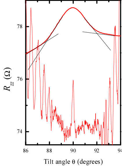
Figure 4. Peaks in the interplane resistance R_{zz} (proportional to \rho_{zz} ) close to \theta = 90^\circ in \lambda -(BETS) 2 GaCl 4 (thick line; T = 1.4 K, B = 30 T; present work) and \kappa -(BEDT-TTF) 2 Cu(NCS) 2 (fine line; T = 520 mK, B = 42 T; reference [30]). In the case of \kappa -(BEDT-TTF) 2 Cu(NCS) 2 , the rapid oscillations at the edges of the figure are angle-dependent magnetoresistance oscillations (AMROs). The fine lines superimposed on the \lambda -(BETS) 2 GaCl 4 data show how the full width of the peak is defined.
