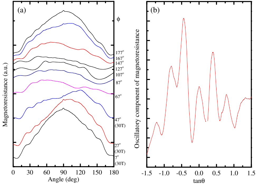
Figure 2. (a) Magnetoresistance of a \lambda -(BETS) 2 GaCl 4 crystal as a function of \theta , the angle between the applied magnetic field and b^* . Data are shown for a number of different \phi -angles (listed on the right of the figure), where \phi is azimuthal angle between the plane of rotation and the b^*c -plane. The lowest three traces were recorded at 30 T; the rest of the data were acquired at 27 T. AMROs are observed as gentle oscillations of the resistance, periodic in \tan\theta ; the small peak at 90^\circ is due to the presence of a small number of closed quasiparticle orbits on the warped Fermi-surface sections. (b) An illustration of the method of locating the AMRO resistance maxima ( \phi = 7^\circ data from (a)). The slowly varying background magnetoresistance has been fitted to a fourth-order polynomial in \theta and subtracted from the experimental data, leaving the oscillatory component. Peaks periodic in \tan\theta are plainly visible.
