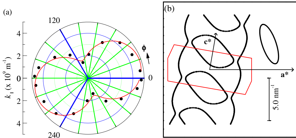
Figure 3. (a) The locus of k_{\parallel} versus azimuthal angle \phi derived from fits of equation (2) to the AMRO data. Data are points and the curve is a fit to equation (3) with the parameters k_x = 4.86 \pm 0.08 \text{ nm}^{-1} , k_y = 1.63 \pm 0.01 \text{ nm}^{-1} , \xi_{\text{inc}} = 19^\circ \pm 5^\circ and b' = 18.4 \text{ \AA} . (b) The experimental cross-sectional shape and orientation of the Q2D Fermi-surface pocket, shown alongside (and to the same scale as) the Brillouin zone, reciprocal-lattice vectors \mathbf{a}^* , \mathbf{c}^* and calculated Fermi surface of reference [15]. The pocket is described by the parameters k_x = 2.43 \pm 0.04 \text{ nm}^{-1} , k_y = 0.815 \pm 0.005 \text{ nm}^{-1} , \xi_{\text{inc}} = 19^\circ \pm 5^\circ and b' = 2 \times 18.4 \text{ \AA} \approx 36.8 \text{ \AA} (see the text and equation (3)).
