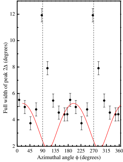
Figure 5. Full widths of peaks in \rho_{zz} close to \theta = 90^\circ for \lambda -(BETS) 2 GaCl 4 (points) plotted as a function of \phi . The curve is given by equations (4), (5) and (6), with t_{\perp} = 0.21 meV. Note that we have chosen to fit data for ranges of \phi at which the Q2D pocket is expected to be the sole provider of closed orbits for in-plane magnetic fields; i.e. we avoided field orientations close to -\mathbf{a}^* ( \phi = 90^\circ ) and \mathbf{a}^* ( \phi = 270^\circ ) (dashed lines) at which the Q1D sheets might also be expected to provide closed orbits in an in-plane field (see figure 3(b))
