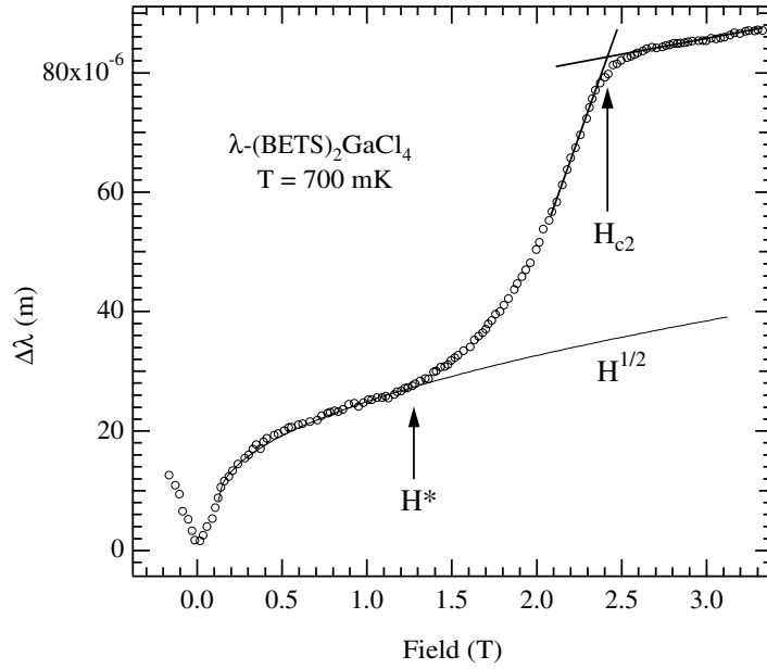
Figure 8. The change in penetration-depth signal versus field for \lambda -(BETS) 2 GaCl 4 at 700 mK. The deviation from the Campbell penetration-depth behaviour is indicated as H^* while the saturation of the \Delta\lambda signal indicates H_{c2} , determined from the straight-line intercepts.
